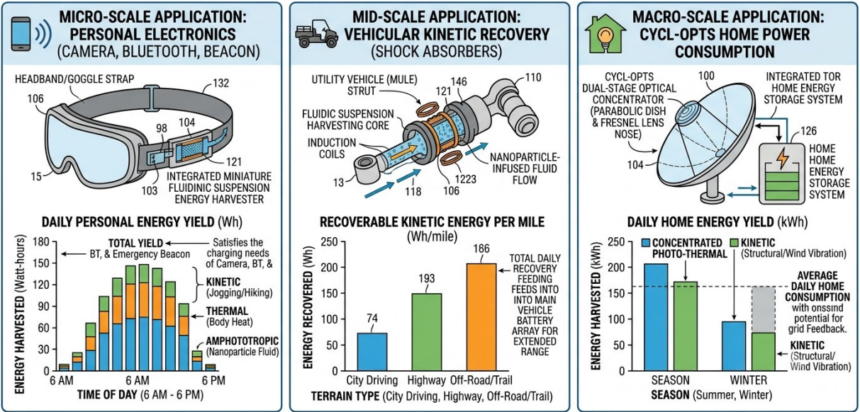
FIGURE X: MULTI-MODAL ENERGY HARVESTING SCALES & DAILY YIELD COMPARISON.
