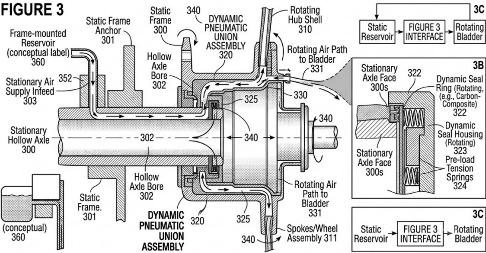
FIGURE 3: DYNAMIC PNEUMATIC TRANSFER INTERFACE (ROTARY AIR UNION)
